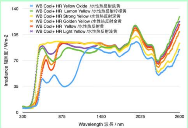
Reflectance of Yellow colorants (masstone) 黄色浆的热反射比 (本色)
